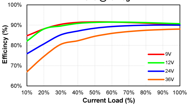
ECLB60W-24S33 Eff Vs Io @25 Deg. C
