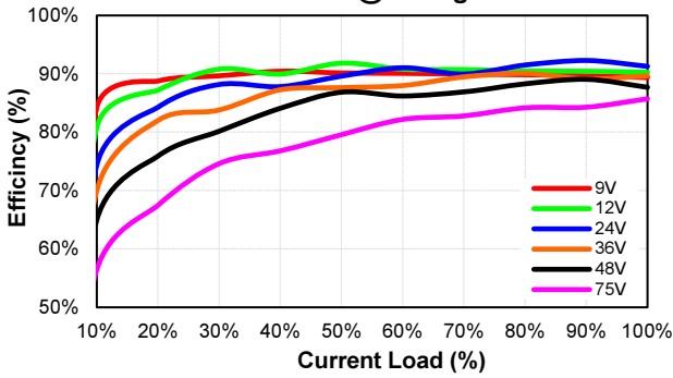
CQB50W8-36S48 Eff Vs Io @25 Deg. C
