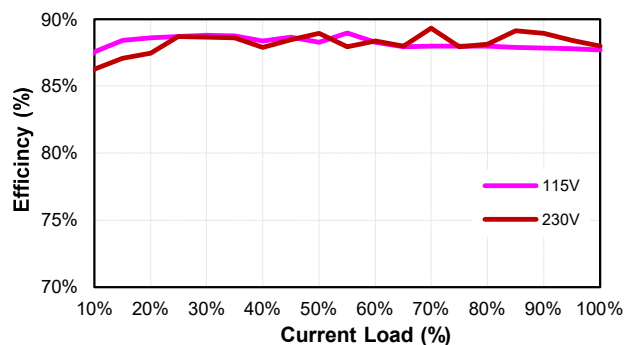
TR30RDM240 (Eff Vs Io)
