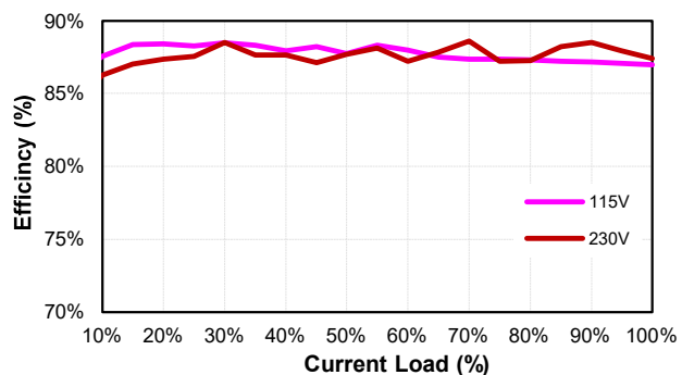
TR30RDM180 (Eff Vs Io)
