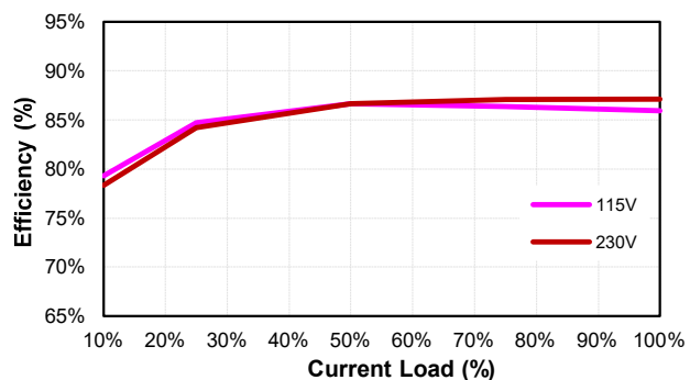
TR30RDM240-PD (20V Eff Vs Io)
