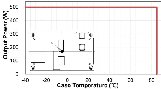
Output Power vs Case Temperature (Tc)
