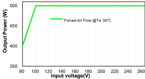
Output power & Input voltage
