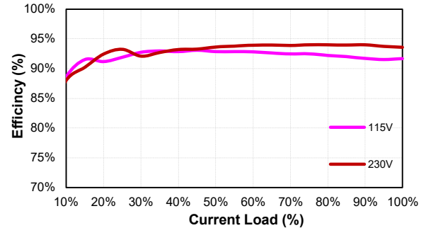
CFM500M180 (Eff Vs Io)
