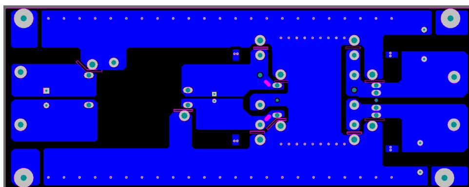
MF20D075P For Half Brick, Quarter Brick and Eighth Brick PCB Bottom Layout
