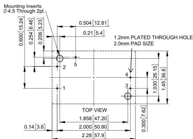
MF20D075P PCB Footprint
