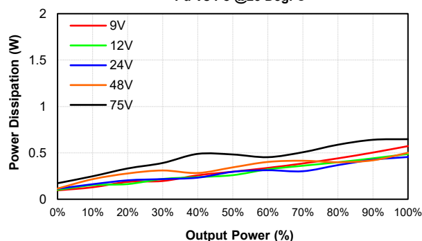
EC3SAW8-48S15P Pd Vs Po @25 Deg. C
