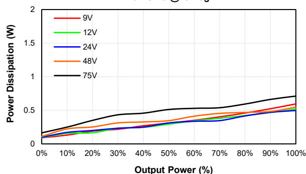
EC3SAW8-48S12P Pd Vs Po @25 Deg. C
