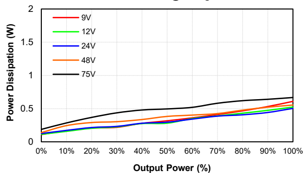
EC3SAW8-48D12P Pd Vs Po @25 Deg. C
