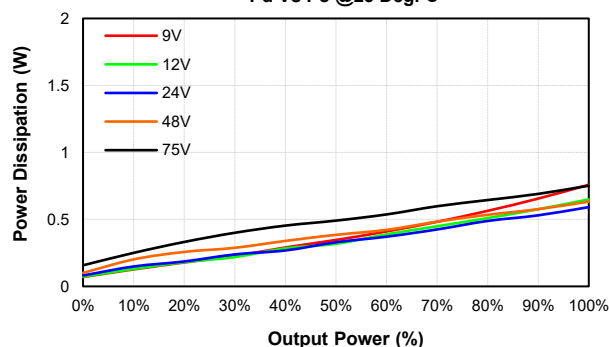
EC3SAW8-48D05P Pd Vs Po @25 Deg. C
