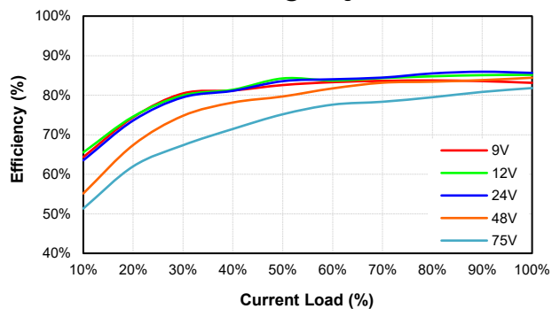
EC3SAW8-48D12P Eff Vs Io @25 Deg. C
