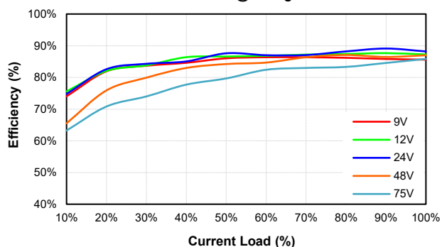
EC4SAW8-48D15N Eff Vs Io @25 Deg. C
