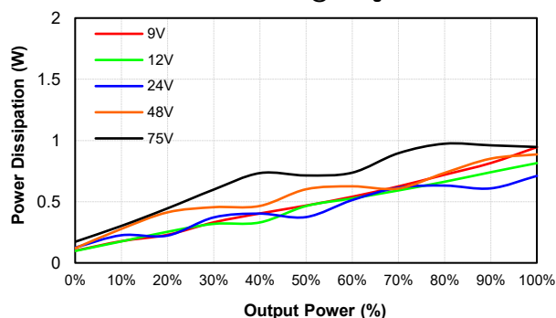
EC4SAW8-48S12N Pd Vs Po @25 Deg. C
