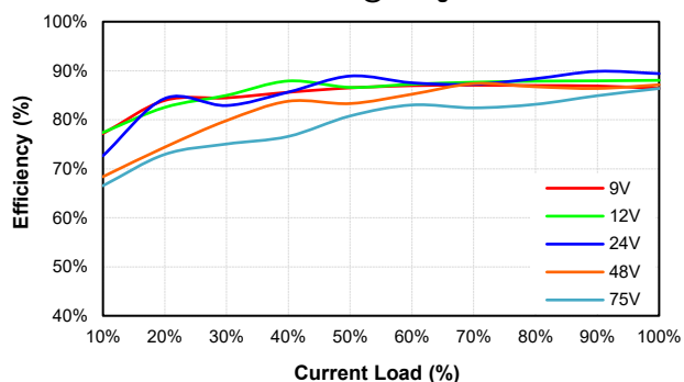
EC4SAW8-48S12N Eff Vs Io @25 Deg. C
