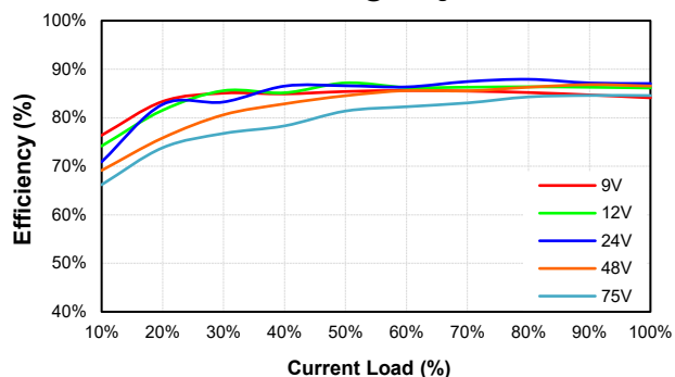
EC4SAW8-48D12N Eff Vs Io @25 Deg. C
