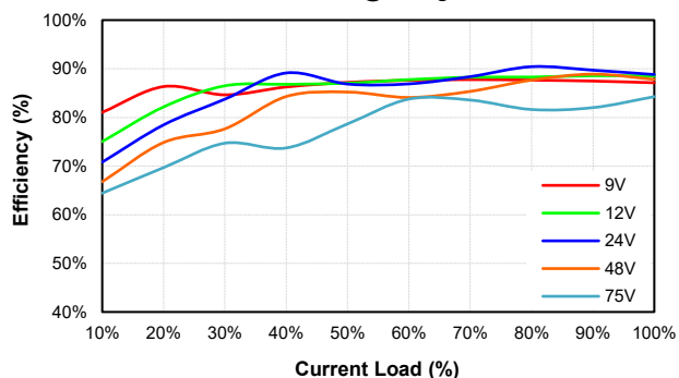
EC4SAW8-48S15N Eff Vs Io @25 Deg. C
