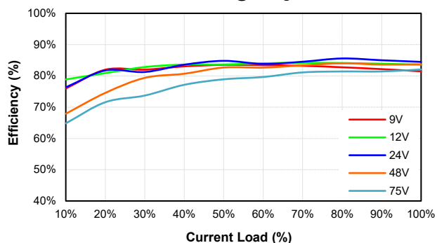
EC4SAW8-48S05N Eff Vs Io @25 Deg. C
